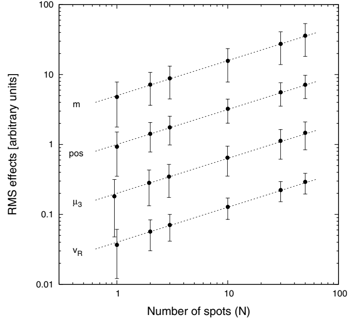
Fig. 2. Results of Monte Carlo simulations of rotating stars with different numbers ( N ) of spots, all the same size ( A = 0.0025 ). The different graphs refer to (from top to bottom) \sigma_m , \sigma_{\text{pos}} , \sigma_{\mu_3} and \sigma_{v_R} , expressed on an arbitrary scale; the dots and error bars show the mean value and dispersion of the \sigma values for a set of simulations with given N . The dashed lines have slope 0.5, corresponding to \sigma \propto \sqrt{N} .
