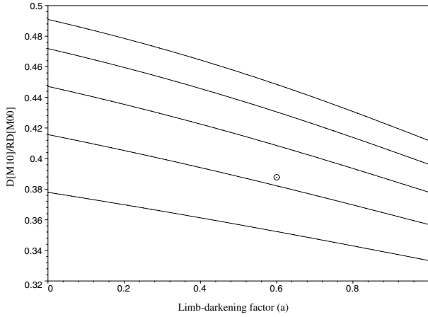
Fig. A.1. The scaling factor D[M_{10}]/RD[M_{00}] from Eq. (A.34) between the expected dispersions in photocentre position and total stellar flux, plotted as a function of the limb-darkening parameter a and the parameter for the centre-to-limb variation of surface structure contrast ( c ). The different curves represent, from top to bottom, c = -1, -0.5, 0, 0.5, 1 . The solar symbol indicates the typical value for solar granulation in white light, a = 0.6 and c = 0.4 .
